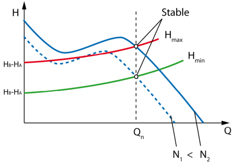
VarSpeed Machine
